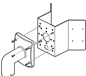
MOUNT POINT 2 Multi Sensor Wall Bracket
