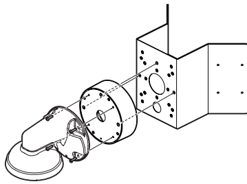
MOUNT POINT 3 Dome Camarea Wall Bracket & Wall Junction Bracket
