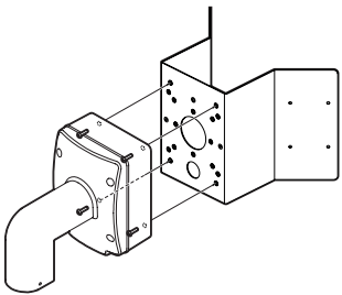
MOUNT POINT 1 PTZ Wall Junction Bracket
