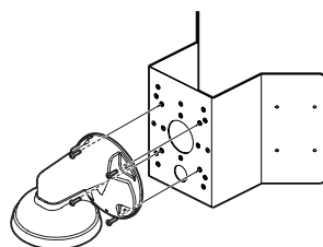
MOUNT POINT 4 Dome Camarea Wall Bracket
